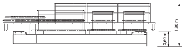
Cross frame
