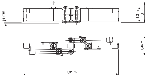
Cross frame
