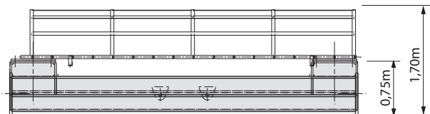
Cross frame
